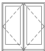
FIBERGLASS DOOR THERMATRU SS118 DOUBLE ACTIVE HINGED 6-0x6-8 FULL GLASS 7 1/2 JAMB
