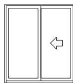
ATRIUM SLIDER 6-0x6-8 FULL VINYL FULL GLASS NO EXTENSION JAMBS WITH SCREEN
