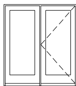
CONSTRUCTION STEEL DOOR THERMATRU PC118 CENTER HINGED SINGLE ACTIVE 6-0x6-8 FULL GLASS 6 9/16 JAMB
